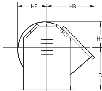
FIELD ADJUSTABLE
