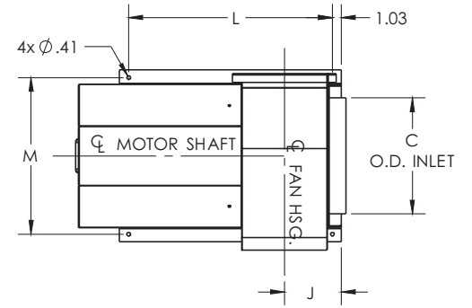
FOUNDATION PLAN
