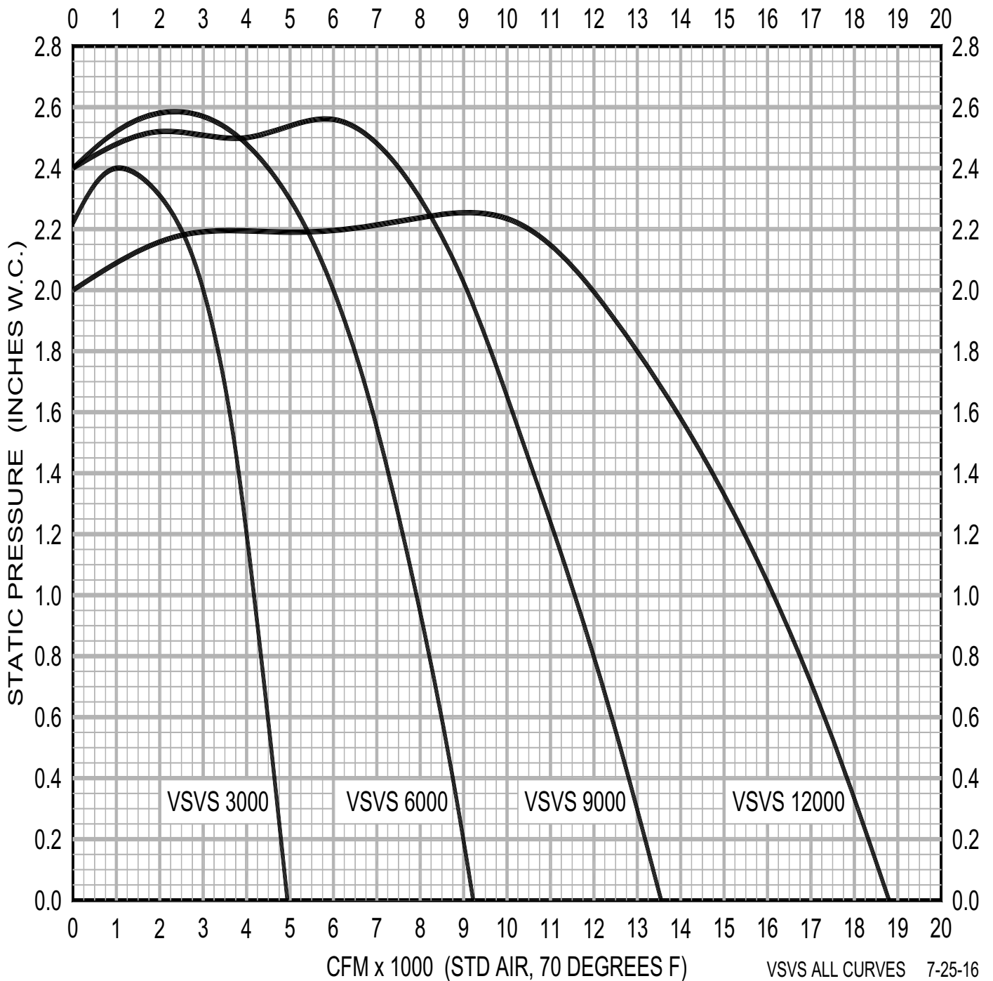
VSVS PERFORMANCE CURVES
